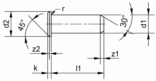
Form A - without transverse hole / continued
